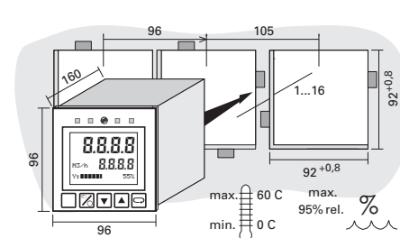
Fig. 3 Dimensions (in mm):
