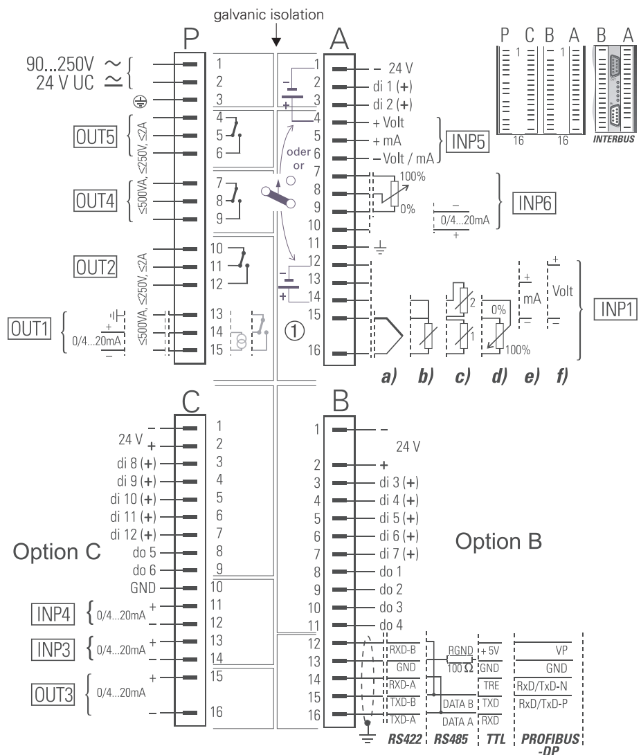
Fig. 1 Electrical connections
