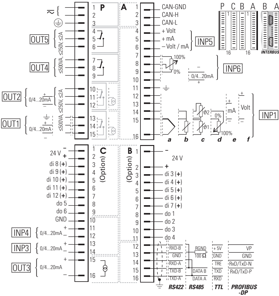
Fig. 5: Communication functions in the KS 98+
