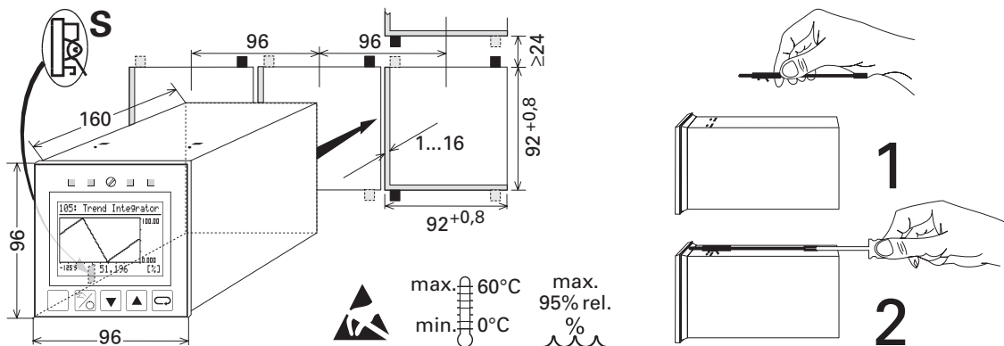
Fig. 6: Overall dimensions
